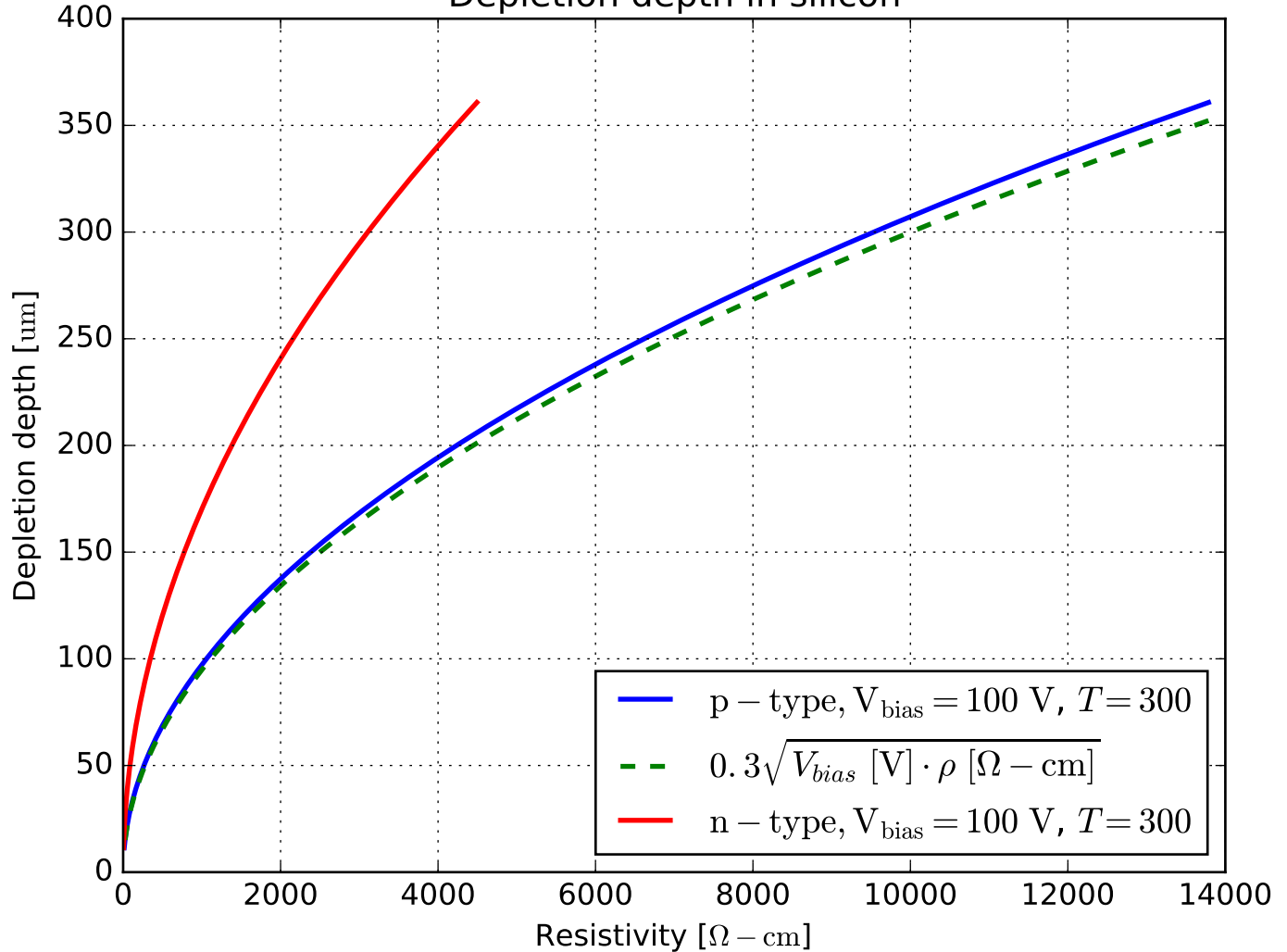
Depletion depth in silicon
